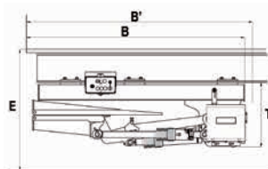
Quick fitting for semi-trailer 1 fold platform
